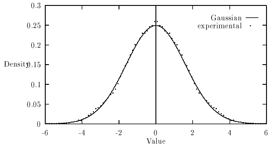
Figure 4: Function 4, Q=10423507 , NGRP=5
