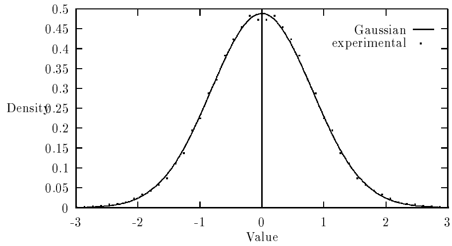
Figure 5: Function 5, Q=10423507, NGRP=5
