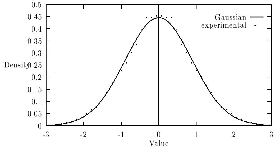
Figure 1: Function 1, Q=10423507 , NGRP=5
