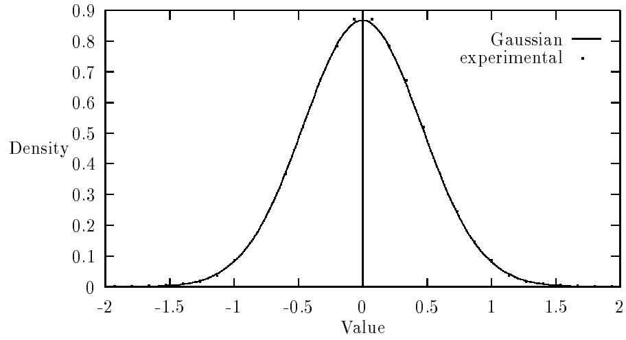
Figure 3: Function 3, Q=10423507 , NGRP=5
