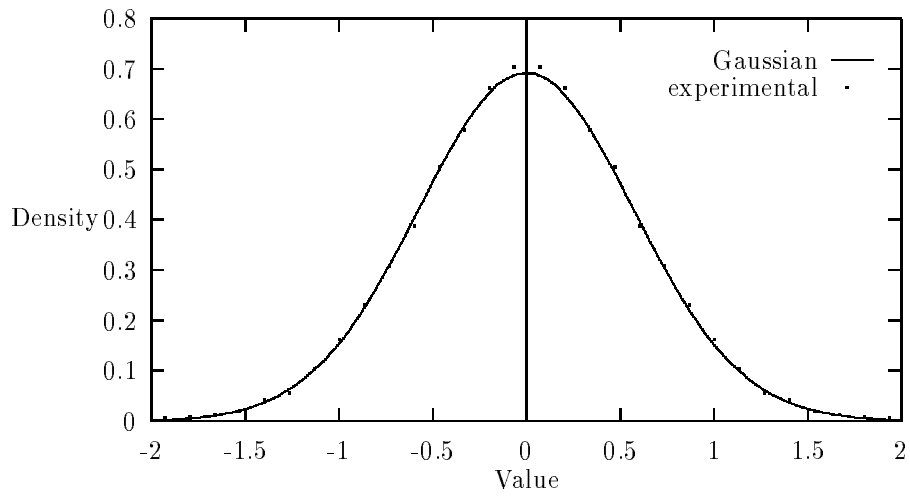
Figure 2: Function 2, Q=10423507 , NGRP=5
