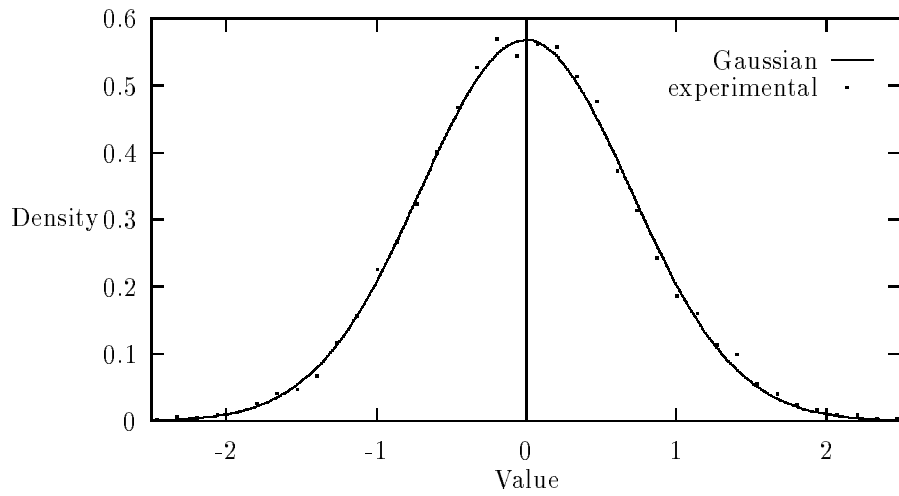
Figure 8: Function 8, Q=10423507, NGRP=5
