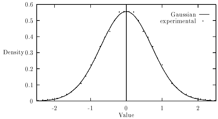
Figure 6: Function 6, Q=10423507, NGRP=5
