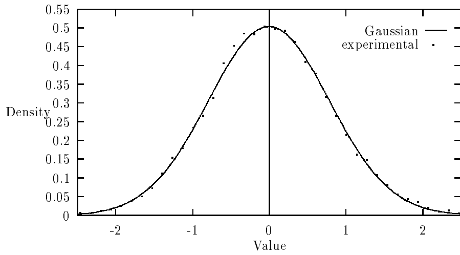
Figure 7: Function 7, Q=10423507, NGRP=5
