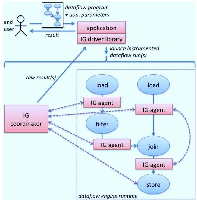
Figure 1: Instrumented dataflow.
