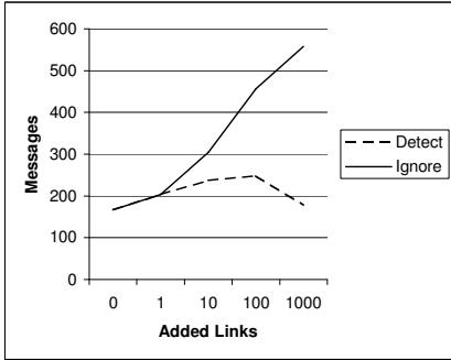
Figure 12. Effect of Cycles
