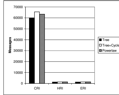
Figure 14. Updates and Network Topology
