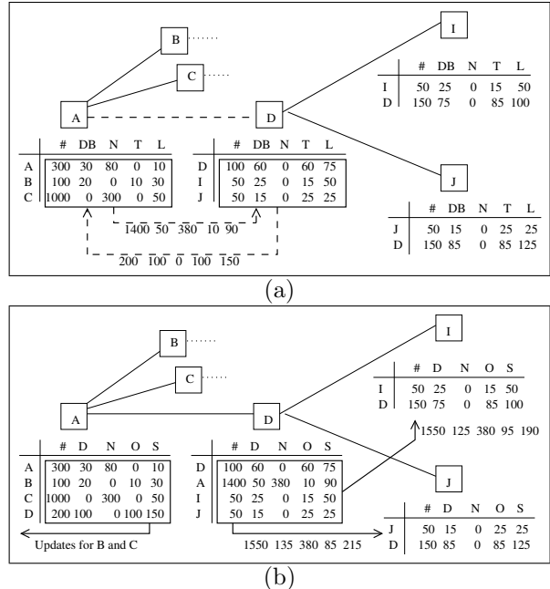
Figure 5. Creating a Routing Index
