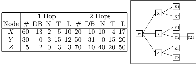
Figure 6. A sample Hop-count RI for node W
