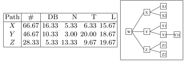
Figure 7. A sample Exponential Routing Index for Node W
