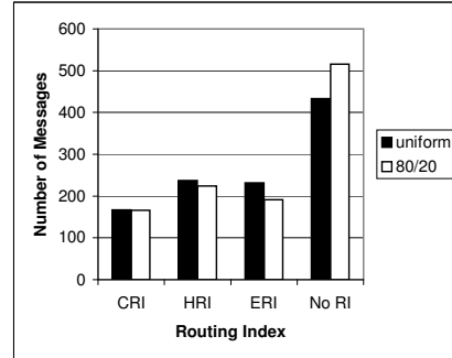
Figure 10. Comparison of CRI, HRI, and ERI
