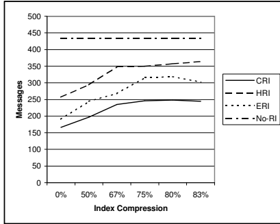
Figure 11. Effect of Overcounts
